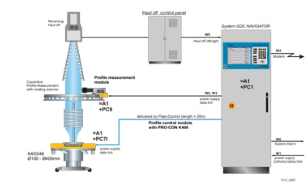
GDCn - PRO-CON K400 PLASTICCONTROL System schematic
